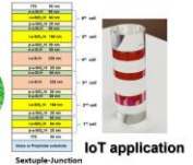
IoT application
